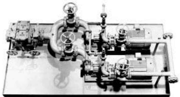
Main and standby 3D-218 fuel pumps on common skid with inlet strainer, discharge relief valves and block valves.
